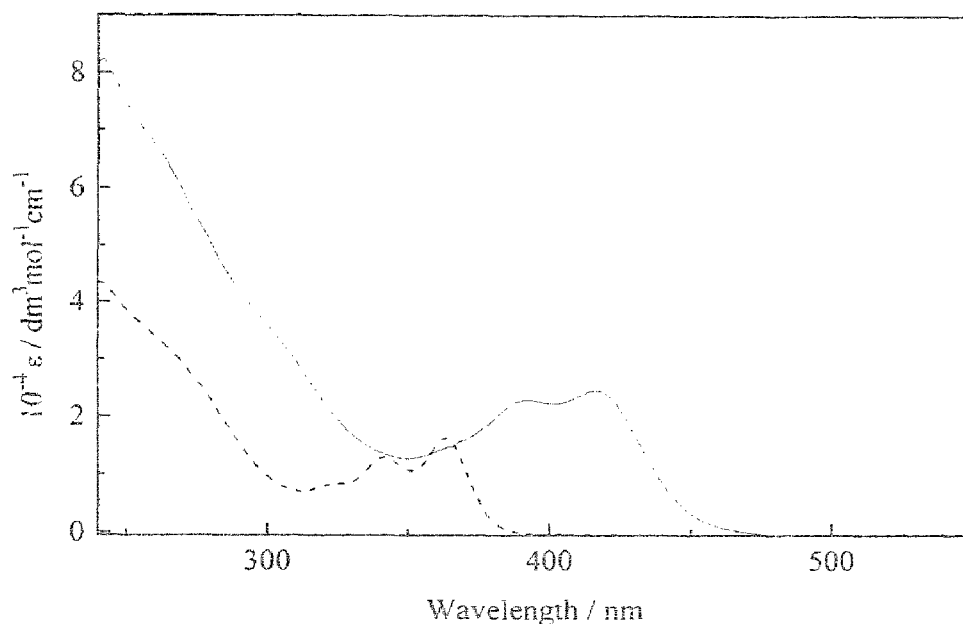
Fig. 6. Electronic absorption spectra of complexes 8 (---) and 9 (····) in \text{CH}_2\text{Cl}_2 .
