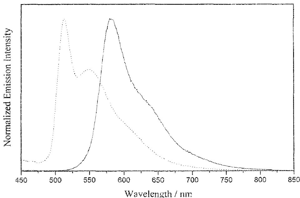
Fig. 7. Solid-state emission spectra of complexes 8 (—) and 9 (---) at room temperature. Excitation wavelength at 350 nm.
