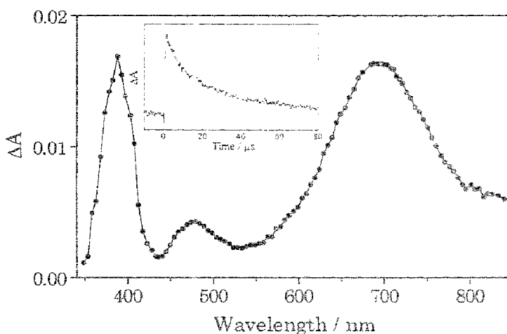
Fig. 5. Transient absorption difference spectrum recorded 10 \mu\text{s} after laser flash excitation for a degassed acetone solution of complex 1 ( 0.27 \times 10^{-3} \text{ mol dm}^{-3} ) and 4-(methoxycarbonyl)- N -methylpyridinium hexafluorophosphate ( 7.93 \times 10^{-3} \text{ mol dm}^{-3} ). The insert shows the decay trace of the transient absorption at 390 nm.
