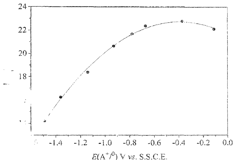
Fig. 8. Plot of \ln k_q + E(\text{A}^{+/0}) for the oxidative electron-transfer quenching of 7 * by pyridinium acceptors in degassed acetone ( 0.1 \text{ mol dm}^{-3} \text{ } ^n\text{Bu}_4\text{NPF}_6 ): (●) experimental, (—) calculated.
