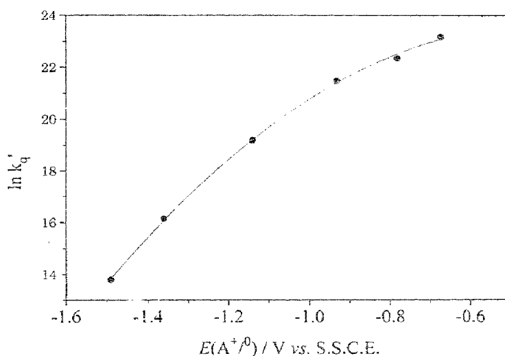
Fig. 4. Plot of \ln k_q' vs E(A^{+•}/^0) for the oxidative electron-transfer quenching of 2^* by pyridinium acceptors in degassed acetone ( 0.1 \text{ mol dm}^{-3} \text{ } n\text{-Bu}_4\text{NPF}_6 ): (●) experimental, (—) calculated.
