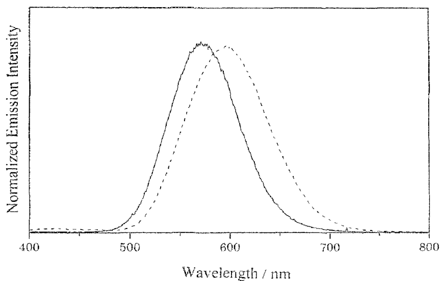
Fig. 1. Solid-state emission spectra of complexes 1 (—) and 2 (---) at room temperature. Excitation wavelength at 350 nm.
