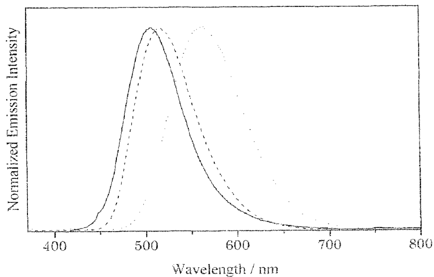
Fig. 2. Solid-state emission spectra of complexes 4 (·····), 5 (---) and 6 (- · - ·) at room temperature. Excitation wavelength at 350 nm.
